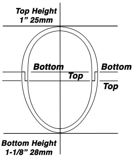
Egg #1 1-3/8" x 2" (34mm x 53mm) Blank size: 1-7/16" x 2-3/4" (37mm x 70mm)
